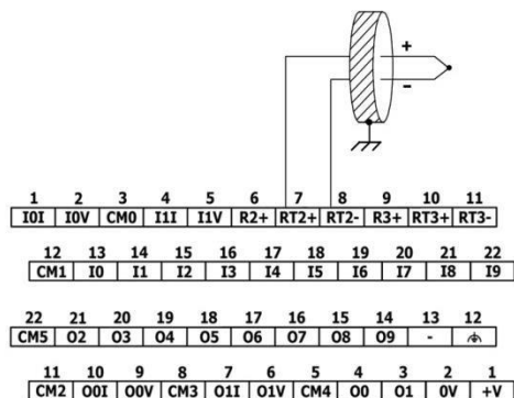
Thermocouple
