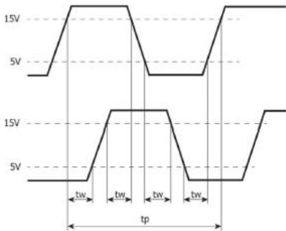
Mode Quadrature
